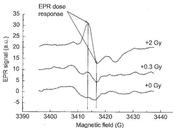
Fig. 2. Evolution of the EPR spectrum with increasing radiation dose for a contemporary US tooth enamel sample.
