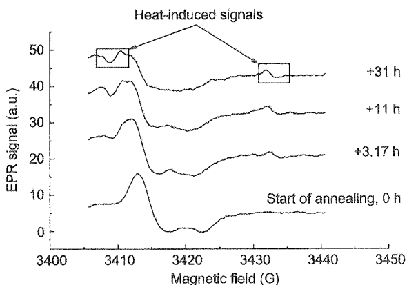
Fig. 1. Time evolution of the EPR spectrum for tooth enamel irradiated to 14 Gy and annealed at 210°C.
