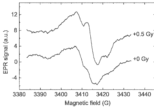
Fig. 3. Pre- and postirradiation (added dose of 0.5 Gy) EPR spectra for an enamel sample prepared from Znamenka tooth no. 4 (Table 1). The reconstructed dose is 170 \pm 30 mGy.
