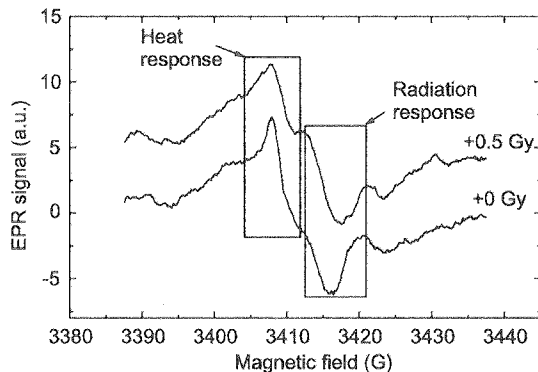
Fig. 4. Pre- and postirradiation (added dose of 0.5 Gy) EPR spectra of an enamel sample prepared from Kainar tooth no. 3 (Table 2). The reconstructed dose is 550 \pm 150 mGy.
