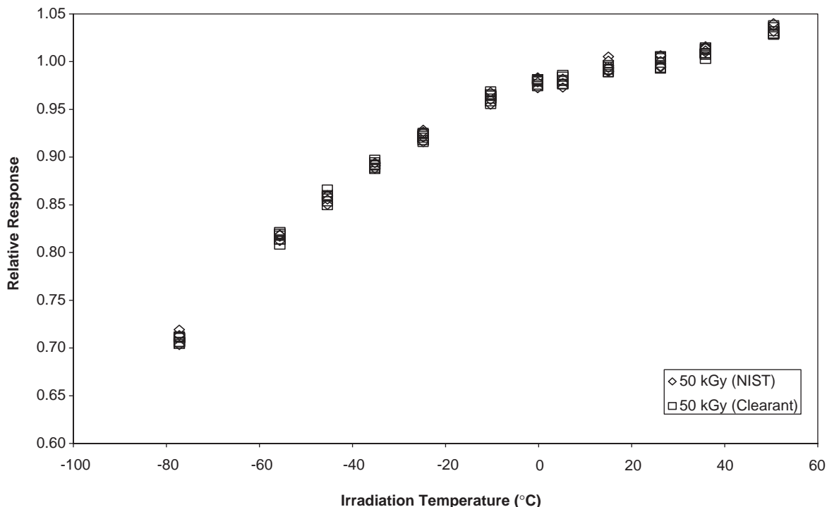
Fig. 3. Dose response relative to that at 25°C for Harwell alanine dosimeters irradiated to an absorbed dose of 50 kGy at fixed temperatures ranging from -77^{\circ}\text{C} to +50^{\circ}\text{C} measured at NIST (ECS106 EPR spectrometer) and Clearant (e-scan EPR spectrometer).
