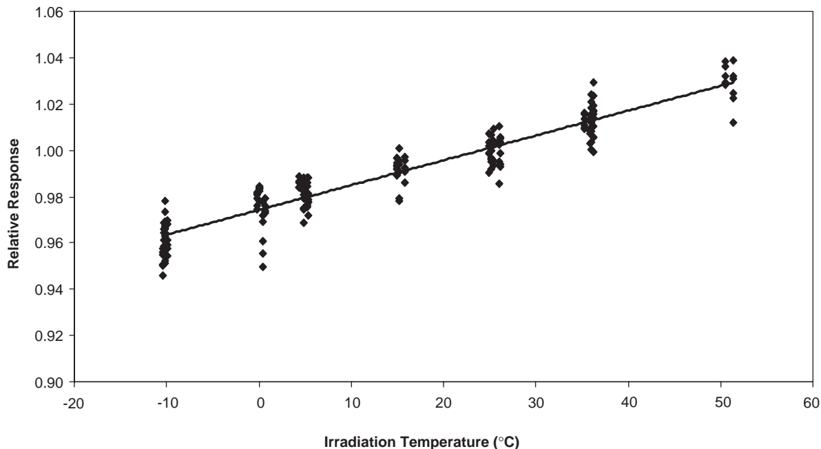
Fig. 1. Dose response relative to that at 25°C for Harwell alanine dosimeters irradiated to absorbed doses of 5, 25, 50, 60, 80 and 100 kGy at fixed temperatures ranging from -10^{\circ}\text{C} to +50^{\circ}\text{C} .
