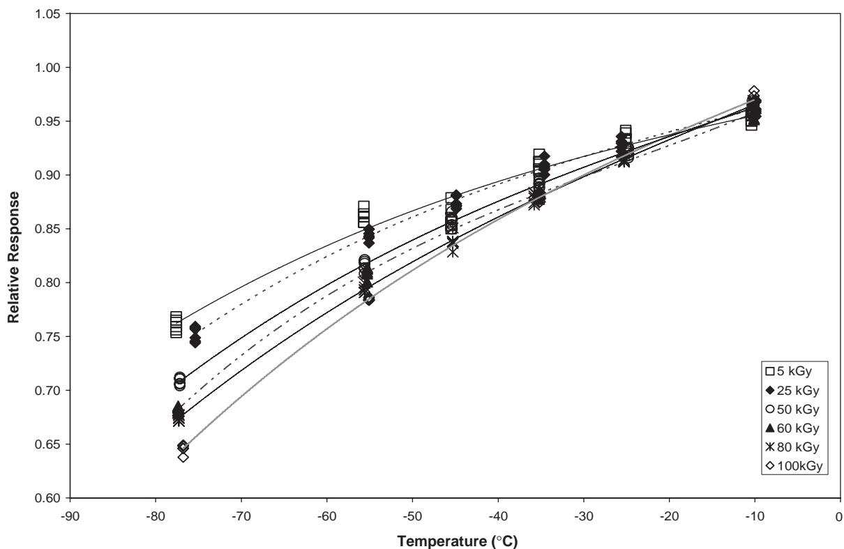
Fig. 2. Dose response relative to that at 25°C for Harwell alanine dosimeters irradiated to absorbed doses of 5, 25, 50, 60, 80 and 100 kGy at fixed temperatures ranging from -77^{\circ}\text{C} to -10^{\circ}\text{C} .
