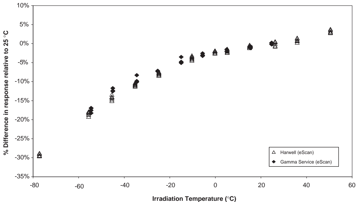
Fig. 5. Relative dose response of Harwell alanine dosimeters irradiated to absorbed doses of 50 kGy at fixed temperatures ranging from -77^{\circ}\text{C} to +50^{\circ}\text{C} (Harwell) and -55^{\circ}\text{C} to +25^{\circ}\text{C} (Gamma Service).
